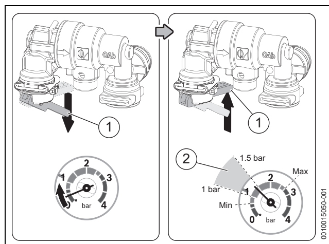
Fig. 5 Keyless filling link
